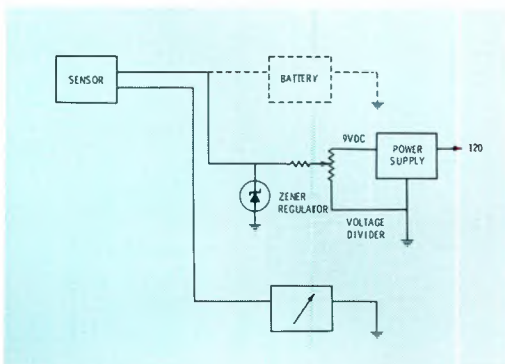
Fig. 4 On the simple system that uses only a battery for supply voltage, you can eliminate the bother of battery replacement. It can be replaced by an AC to DC power supply. If voltage is higher than required, add a resistor voltage divider and a zener diode for regulation.
